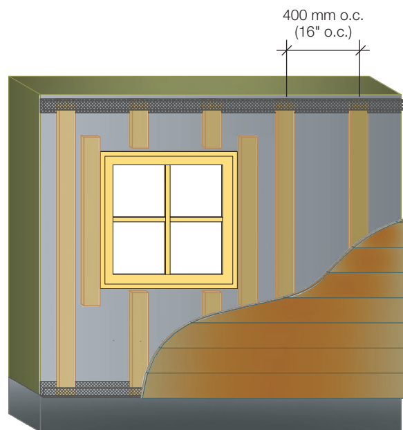
FIGURE 4 • Position of furring strips for horizontal cladding
