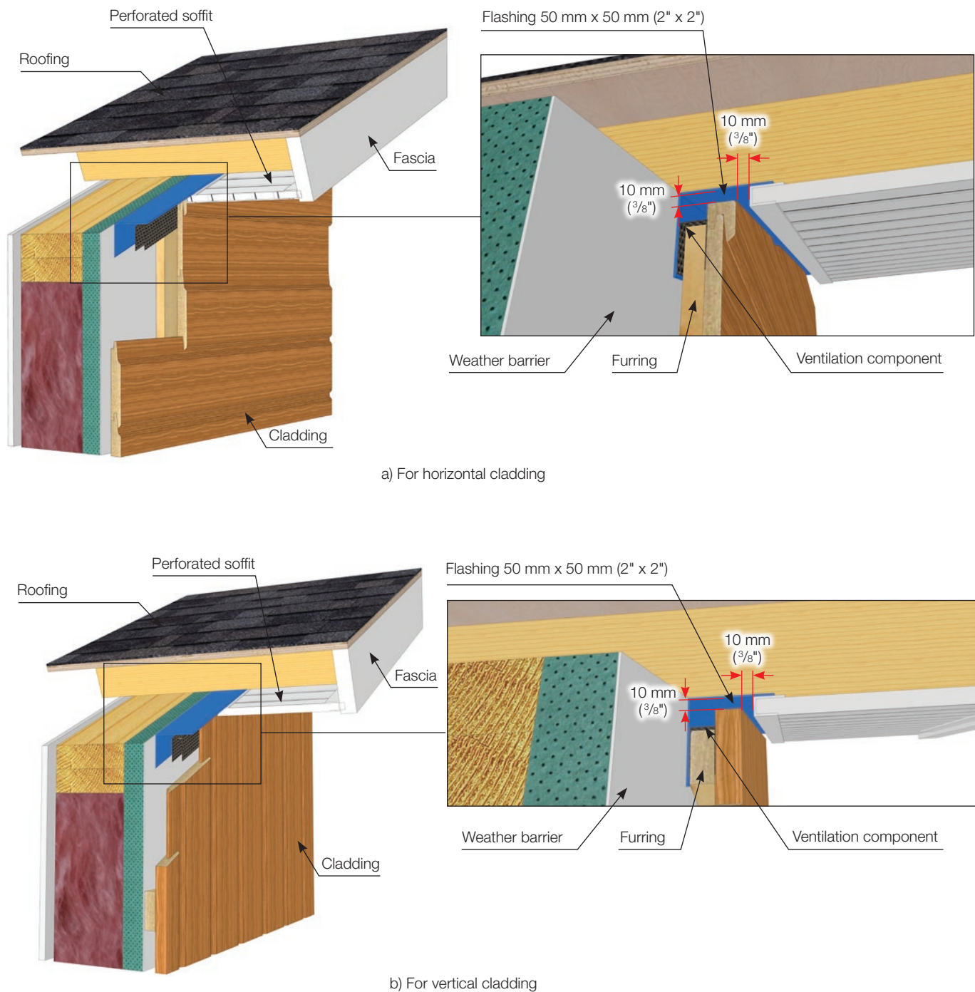
FIGURE 15 • Opening at top of a gable
